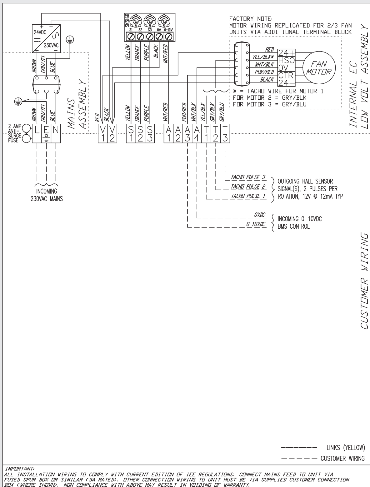
Figure 6. Sample wiring diagram
