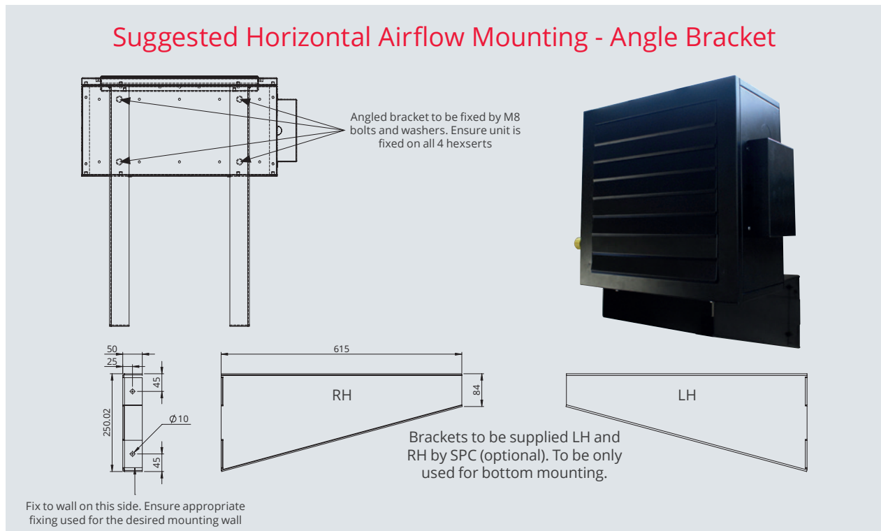
Figure 2. Wall angle bracket fixing
