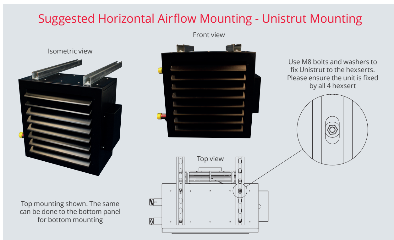
Figure 3. Horizontal unit Unistrut fitting
