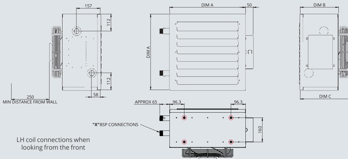
Figure 1. Major dimensions
